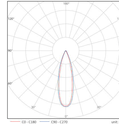
Beam Angle: 30°
